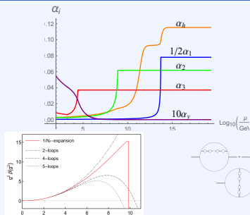
Safe-SM running; resummed g^2 \beta(g^2) versus finite-loop truncations; bubble-chain topologies in the large- N_f expansion.
