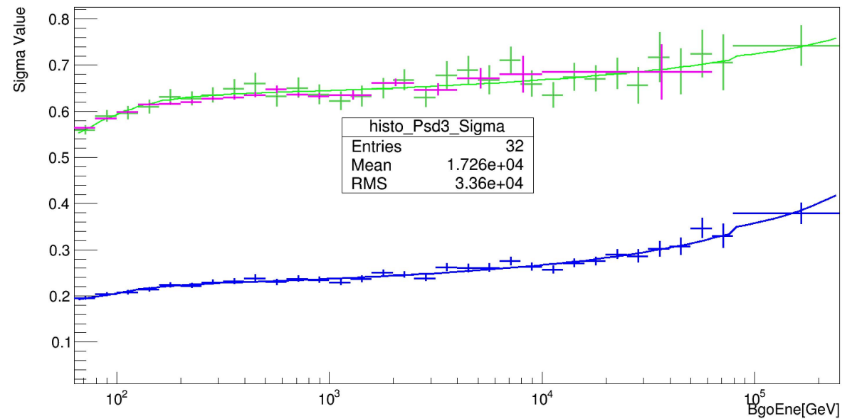
PsdQ_Layer3 Sigma Value
