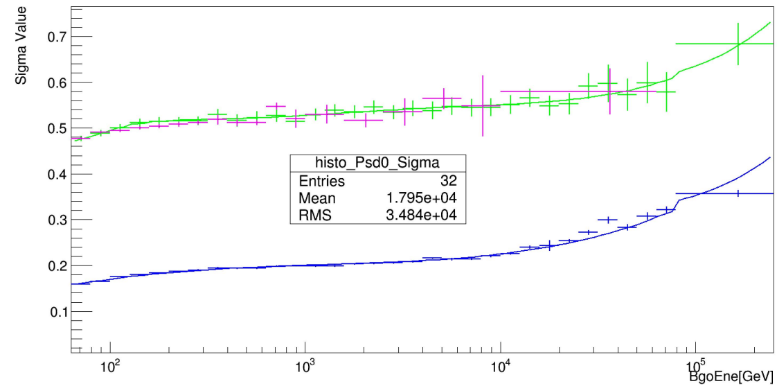
PsdQ_Layer0 Sigma Value
