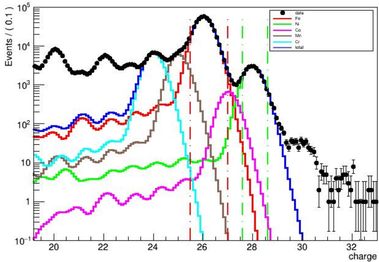
A RooPlot of "charge"
