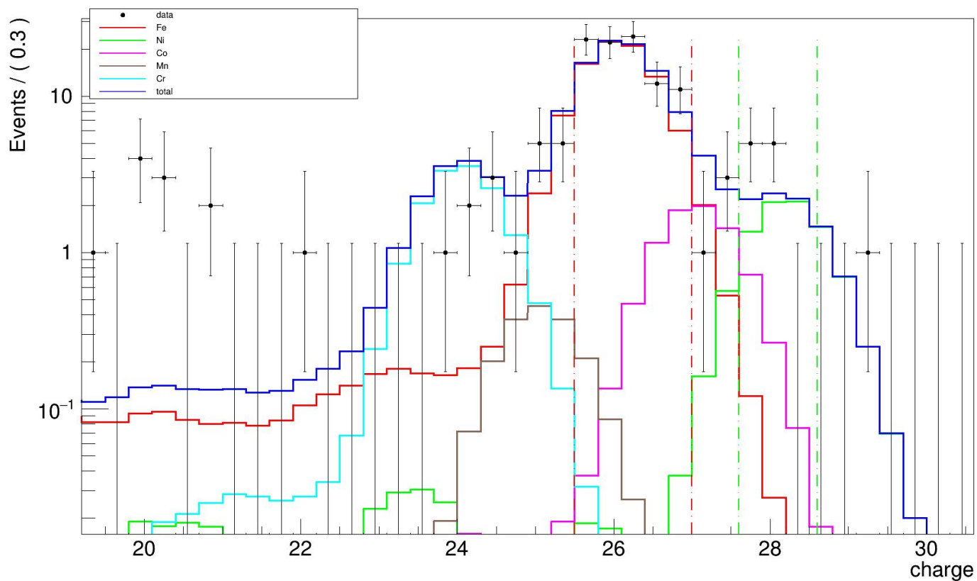
A RooPlot of "charge"
